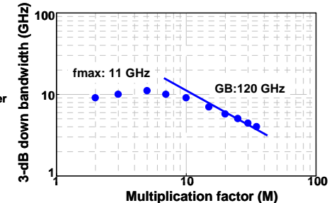
Frequency Response
