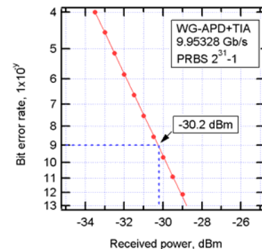
Received Sensitivity
