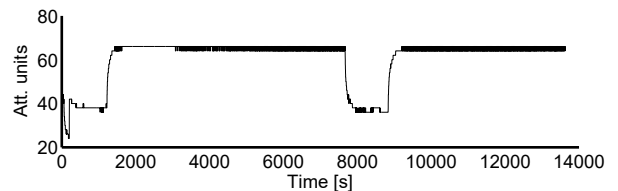
(c) AGC attenuation
