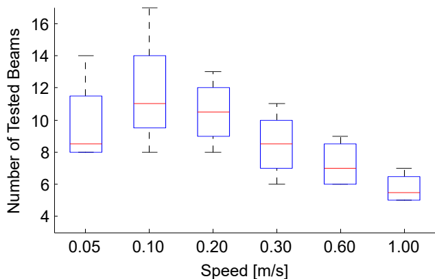
Figure 9: Number of beam tests during blockage
