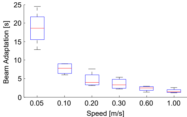
Figure 8: Duration of beam pattern adaptation.
