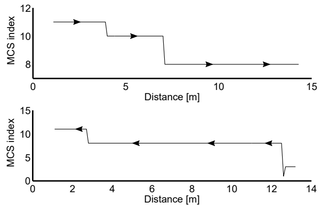
Figure 7: MCS for increasing/decreasing link length
