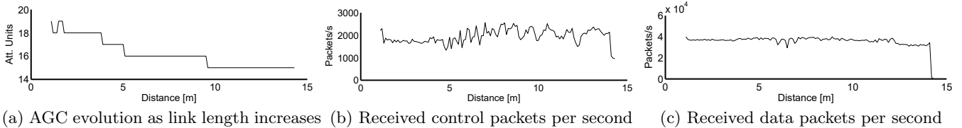
Figure 5: Mobility analysis for a continuously increasing link length.
