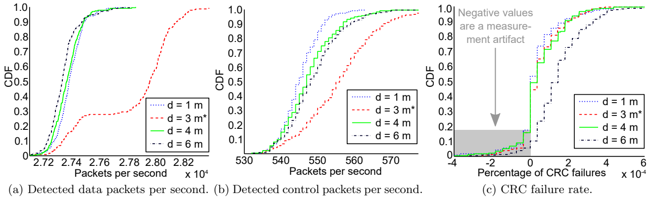
Figure 3: Distance impact. The case for d = 3 meters (marked with *) involved two different MCSs.
