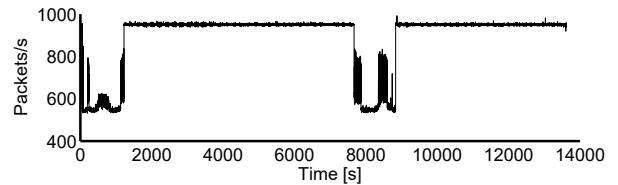
(b) Received physical layer control packets
