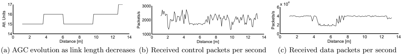
Figure 6: Mobility analysis for a continuously decreasing link length.
