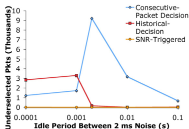
Figure 10: Undersampled packets by the loss-triggered protocols as interference is injected.
