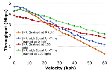
Figure 9: Throughput with multipath-induced fading for SNR-based protocols.
