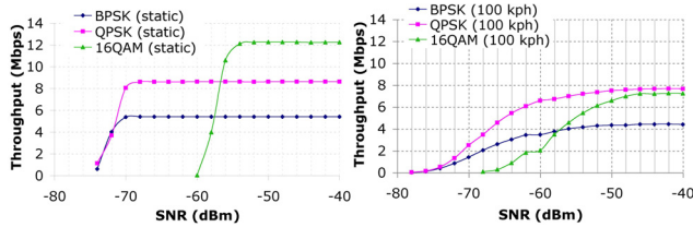
Figure 7: Performance of modulation schemes at 0 kph (left) and at 100 kph (right).
