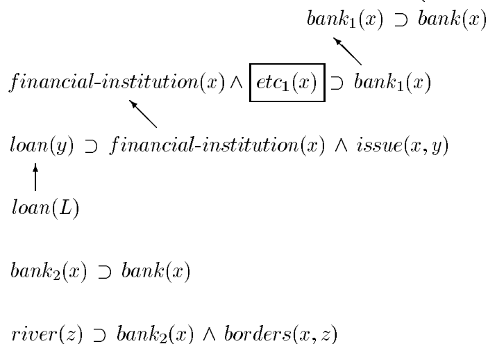
Figure 5: Interpretation of “... the bank.”
