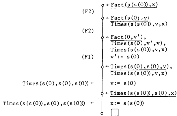
Fig. 1. A computation of the factorial of 2. In each goal statement, the selected procedure call is underlined. The arc, connecting C_i with C_{i+1} is labelled by the procedure used to derive C_{i+1} from C_i . The same arc is labelled by the assignment of terms to variables which is that part of the matching substitution which can be interpreted as passing output from the procedure name to the procedure call.
