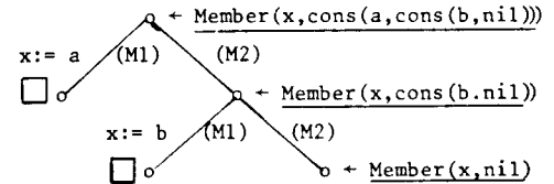
Fig. 2. The space of all computations determined by (M1)-(M3). The space contains two successful computations and one unsuccessfully terminating computation.
