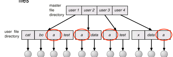
Two-level directory
