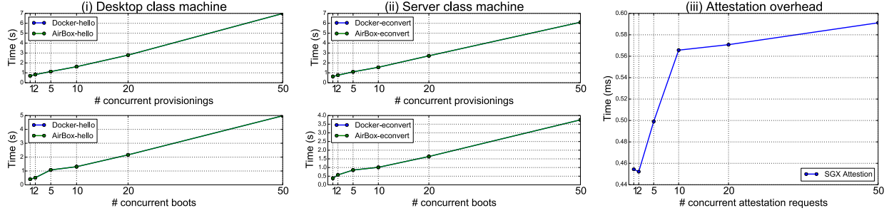
Figure 4: Comparing provisioning time using Docker and AirBox including a hello world and an image inverting application vs. increasing number of simultaneous provisioning requests using (i) desktop class machine and (ii) server class machine; (iii) time spent in attestation command vs. number of simultaneous attestation requests using windows SDK on SGX hardware.
