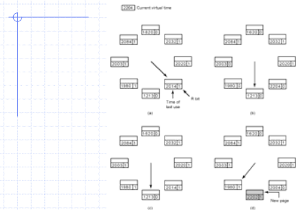
Operation of the WSclock algorithm
