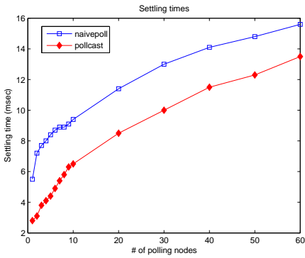
Fig. 2. Settling time
