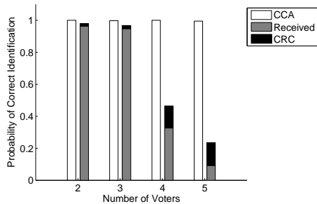
Fig. 1. Collision detection performance
