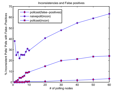
Fig. 4. Polling inconsistencies
