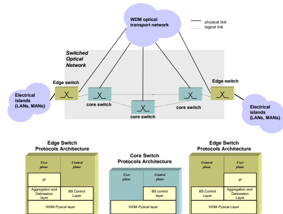
Fig. 1: Optical switched network architecture
