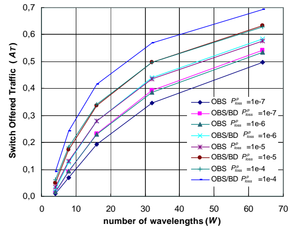
Fig. 6: Switch offered traffic ( A_T ), normalised to W , as function of the number of data wavelengths ( W ) in order to have P_{loss}^p varying from 10^{-7} to 10^{-4} for N=16
