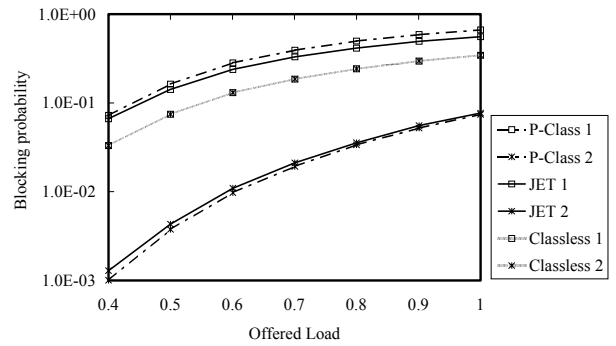
Figure 1. Blocking probabilities of the three mechanisms
