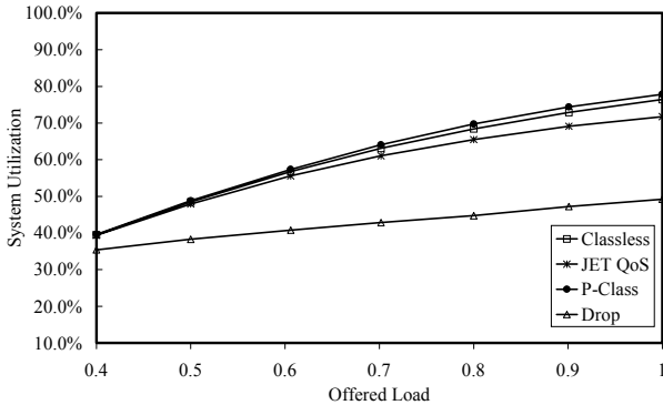
Figure 3. System utilization of the four mechanisms
