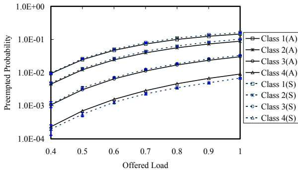
Figure 5 Preempted probability of an accepted call
