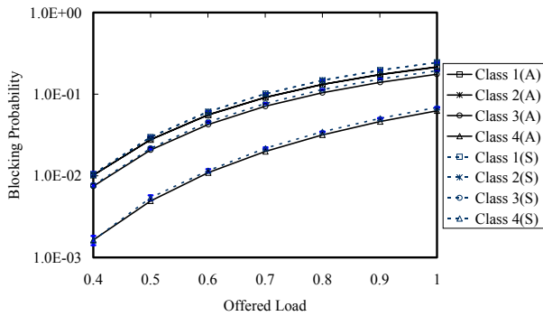
Figure 4. Blocking probability of new bursts
