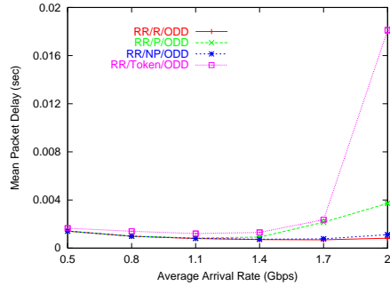
Fig. 8. Mean packet delay
