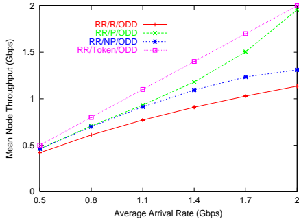
Fig. 4. Mean node throughput
