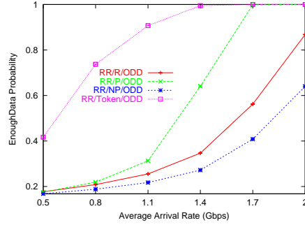
Fig. 7. EnoughData probability
