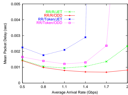
Fig. 11. Mean packet delay
