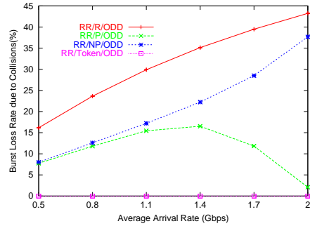
Fig. 5. Burst loss due to collisions
