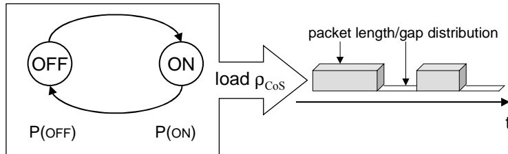
Fig. 3. Source for traffic modelling with strictly alternating ON and OFF states
