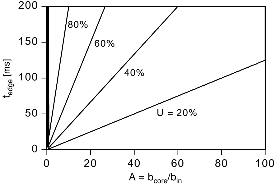
Fig. 7. Bandwidth utilisation, U , as a function of t_{\text{edge}} and A for a round-trip time t_{\text{RTT}} = 5 ms
