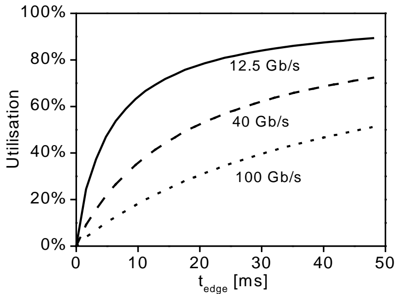
Fig. 6. Utilisation U as a function of t_{\text{edge}} for t_{\text{RTT}} = 5 ms, b_{\text{in}} = 10 Gb/s and b_{\text{core}} = 12.5, 40, and 100 Gb/s
