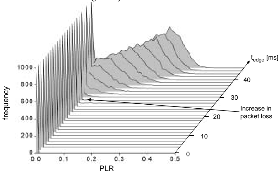
Fig. 5. Graph showing the PLR distribution as a function of edge delay. Significant deviations of the PLR from the mean is observed for Pareto traffic statistics ( \alpha = 1.5 ) at the input for t_{\text{edge}} > 30 ms.
