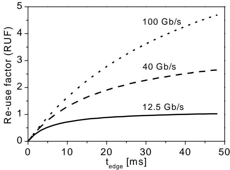
Fig. 8. Wavelength re-use factor RUF as a function of t_{\text{edge}} for t_{\text{RTT}} = 5 ms and b_{\text{core}} = 12.5, 40, and 100 Gb/s
