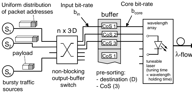
Fig. 2. Edge router model with electronic pre-sorting, non-blocking output-buffered switch and tuneable wavelength section
