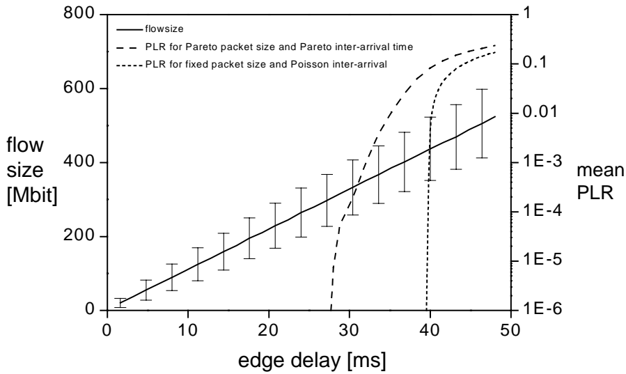
Fig. 4. Simulation results for flow size and PLR as a function of the edge delay for B = 400 Mbit and a mean input bit-rate b_{\text{in}} = 10 Gb/s. Flow size (solid) and a mean PLR for fixed packet, Poisson inter-arrival (dotted) and Pareto packet size, Pareto inter-arrival (dashed) distribution
