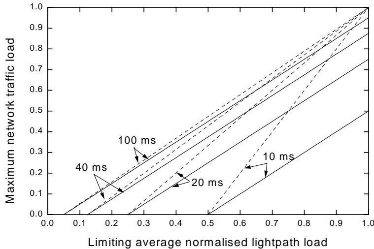
Figure 6. Maximum network traffic load ( \bar{v}_{max} ) vs. limiting average lightpath load ( \bar{\rho}_{lim} ) for different average edge delays ranging from 10 to 100 ms. Solid lines represent the limits for LS-Bursts, and dashed lines those for NS-Bursts.
