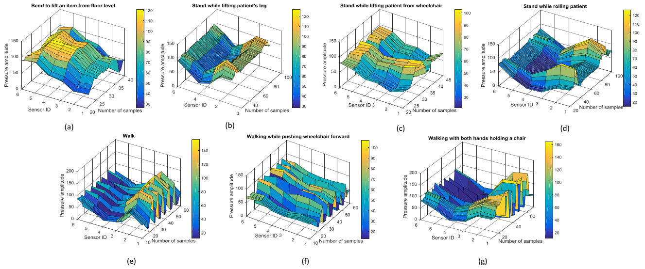
Figure 5. The 3-D visualization of pressure data from Smart Insole 2.0: (a) Bend leg to lift an item from floor level; (b) Stand while lifting patients leg; (c) Stand while lifting patient from wheelchair; (d) Stand while rolling patient; (e) Walk forward; (f) Walk while pushing wheelchair forward; (g) Walk with both hands carrying a chair.
