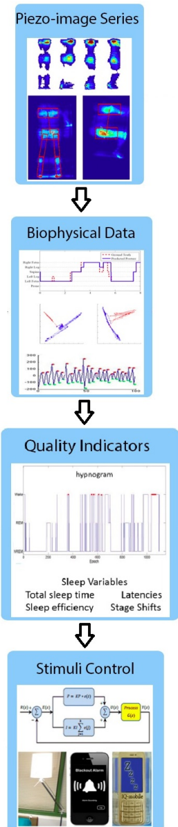
Figure 2: EZwakeup algorithmic flowchart from sensing to controlling
