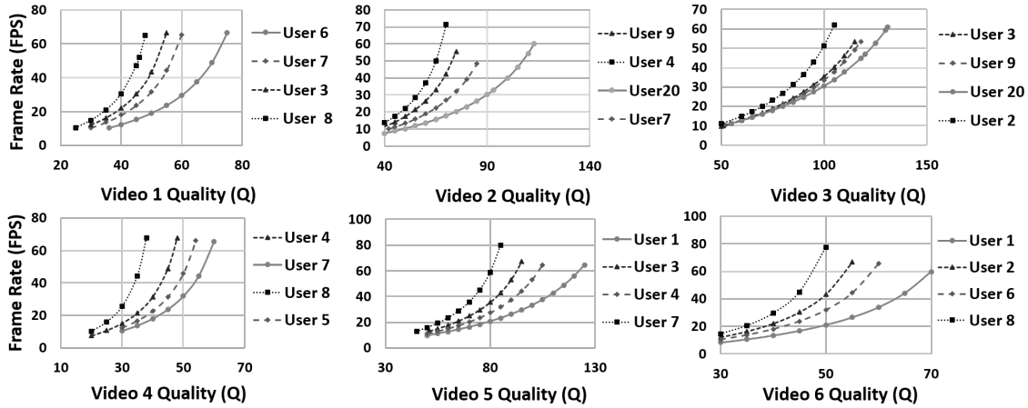
Figure 6: Offline frame rate library generation based on 6 videos and 4 selected users of each video.
