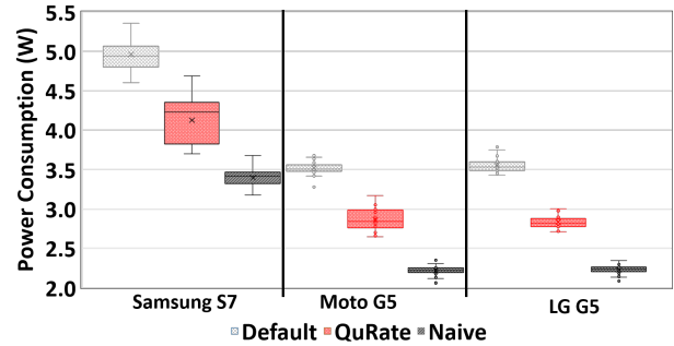
Figure 10: Boxplot of measured average power consumption of Users 10 - 14 watching Videos 1 - 6 for Samsung S7, Moto G5, and LG G5.
