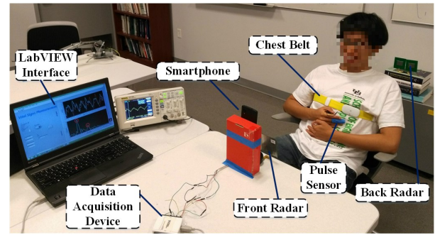
Figure 8: Experimental setup for cardiac motion sensing. A subject is sitting one meter away from both radar sensors, a chest belt and a pulsed sensor is attached to the subject.
