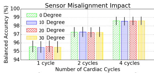
Figure 13: The BAC comparison for misalignment.
