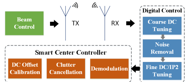
Figure 3: Doppler radar sensor with adaptive DC tuning.
