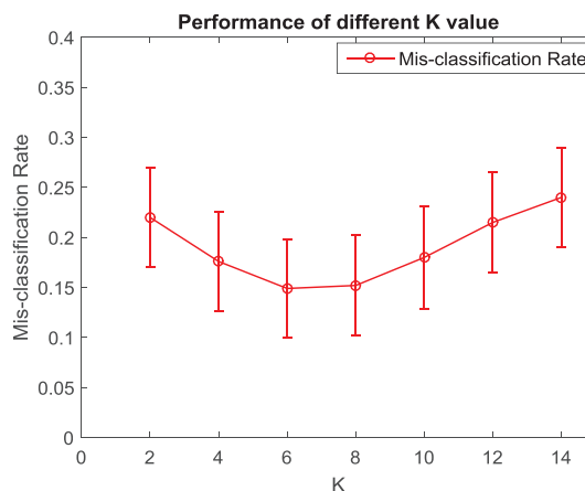
Fig. 12. Performance impact of different K value for action manifold learning.
