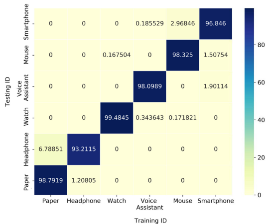
Fig. 17. SonicPrint performance to identify interacting object based on swipe actions.
