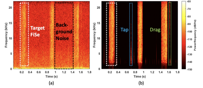
Fig. 6. The spectrogram of (a) original and (b) denoised FiSe from three swipe actions.
