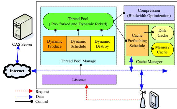
Fig. 5. The UbiCAS Proxy structure.
