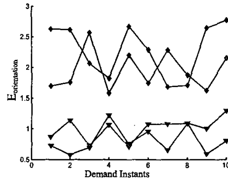
Figure 6. Absolute errors in target's surface normal estimates.
