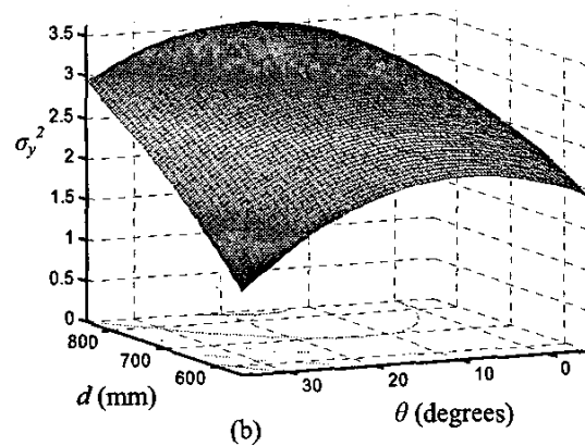
Figure A2. Response surfaces of variances in (a) position and (b) orientation estimation.
