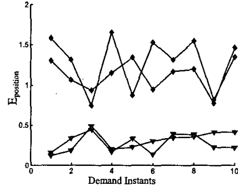
Figure 5. Absolute errors in target position estimates.
