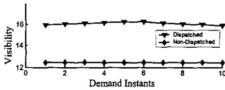
Figure 4. Observed visibility.
