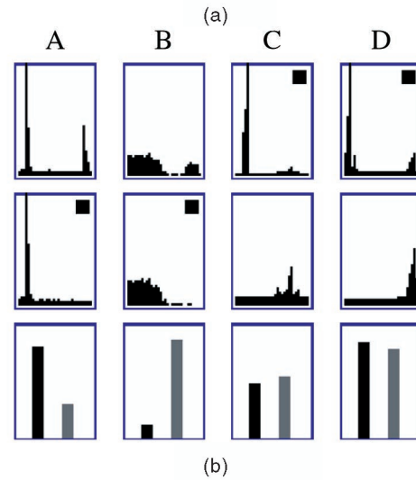
Fig. 9. Local evidence with different convolution kernels. (a) Four points (A, B, C, and D) in the sixth frame of the “garden” sequence (11 frames) are semiocclusion points. (b) Each column corresponds A, B, C, and D, respectively. The first row shows local evidence \Psi_s(x_s, y_s) using convolution kernel w_d(s, d_s, k) . The horizontal and vertical coordinates are disparity and matching probabilities, respectively. The second row shows local evidence \Psi_s(x_s, y_s) using convolution kernel w_f(s, d_s, k) . The last row shows F^- (black) and F^+ (gray). The evidences marked with a black rectangle at the top right corner are computed by our convolution kernel w_a(s, d_s, k) .
