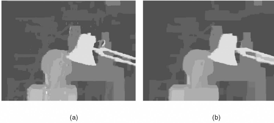
Fig. 12. (a) Result of TV model ( B_O = 2.16 , B_T = 1.01 , B_{DD} = 11.67 ). (b) Result of Gaussian model ( B_O = 2.82 , B_T = 1.58 , B_{DD} = 15.14 ). The results obtained by TV model \rho_p(d_s, d_t) = \frac{|d_s - d_t|}{\sigma_p} and Gaussian model \rho_p(d_s, d_t) = \frac{|d_s - d_t|^2}{\sigma_p} . The parameter \sigma_p is chosen experimentally to produce the best result for each model.
