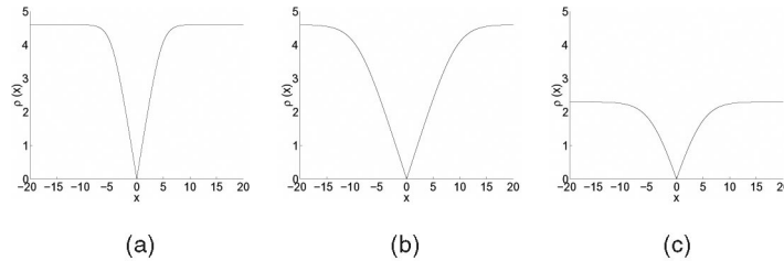
Fig. 2. (a) e = 0.01, \sigma = 1.0 . (b) e = 0.01, \sigma = 2.0 . (c) e = 0.1, \sigma = 2.0 . Robust function \rho(x) = -\ln((1 - e) \exp(-\frac{|x|}{\sigma}) + e) derived from TV model. Parameters \sigma and e , respectively, control the sharpness and the upper-bound of the function.
